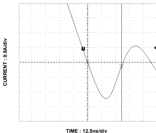
Figure 12. FDS6676S SyncFET body diode reverse recovery characteristic.
