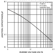
FIG.7-TYPICAL JUNCTION CAPACITANCE PER LEG
