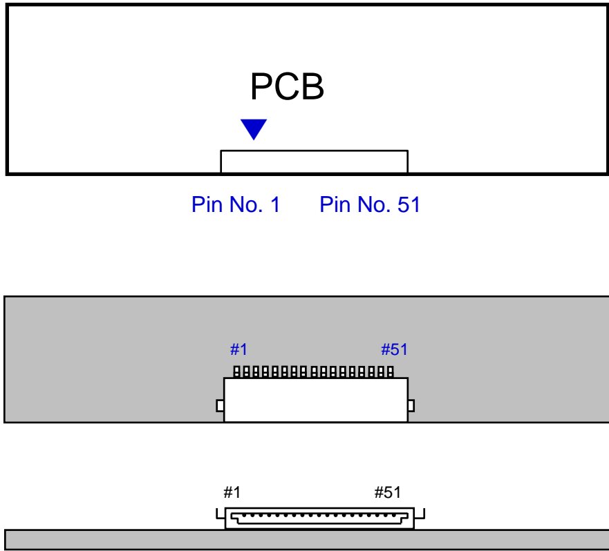
Fig. Connector diagram
