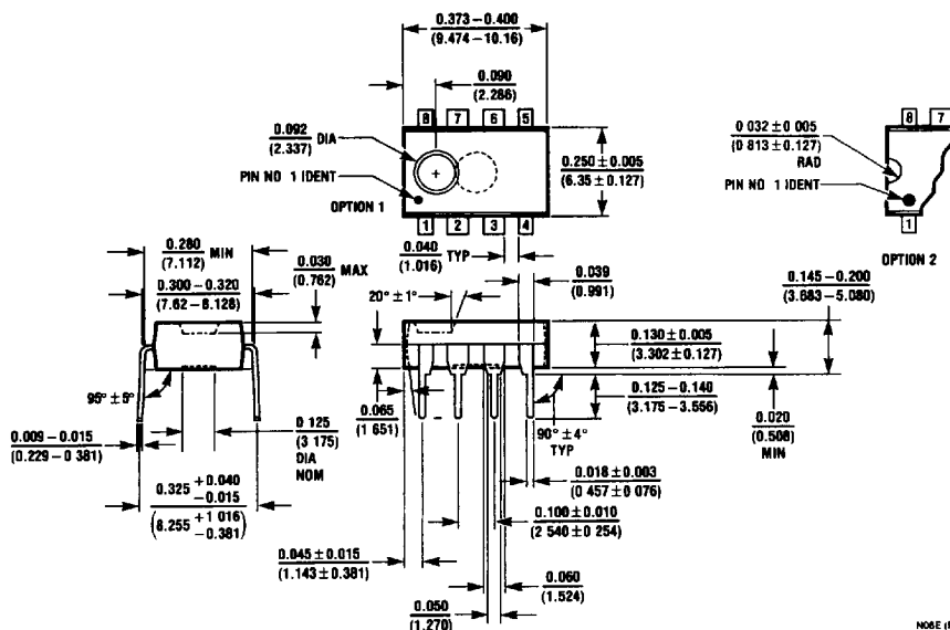
8-Lead Molded Dual-In-Line Package (N) Order Number NM93C46XLZN NS Package Number N08E
