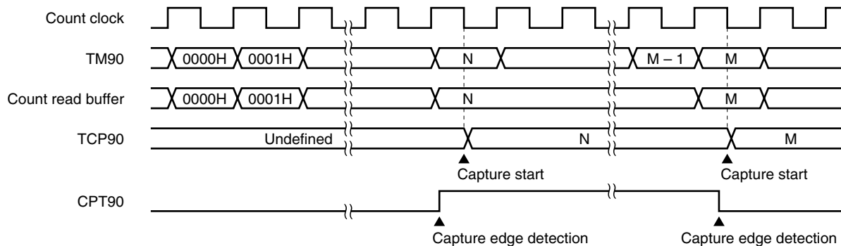
Figure 6-10. Capture Operation Timing (with Both Edges of CPT90 Pin Specified)
