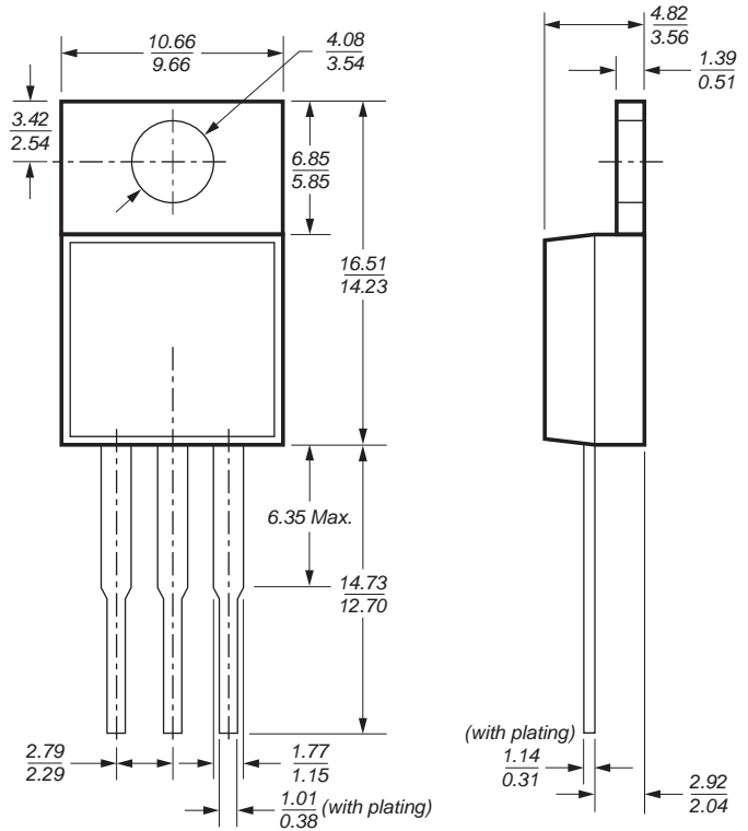
TO-220 Case Outline
