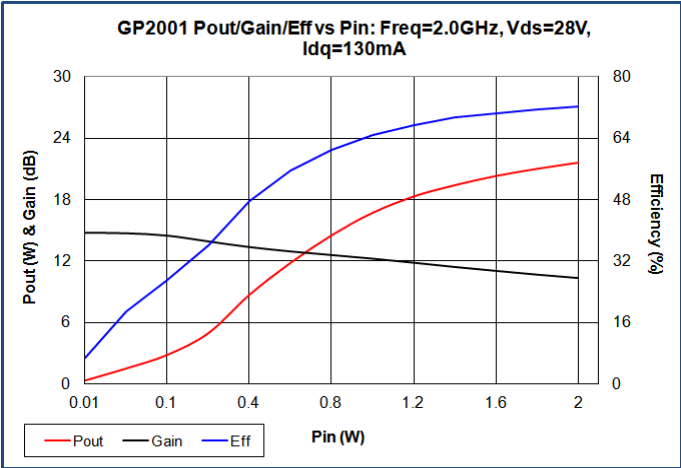
BROADBAND PERFORMANCE
