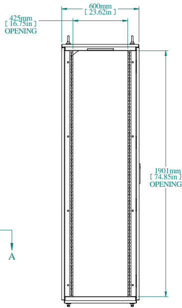
L.S. VIEW
