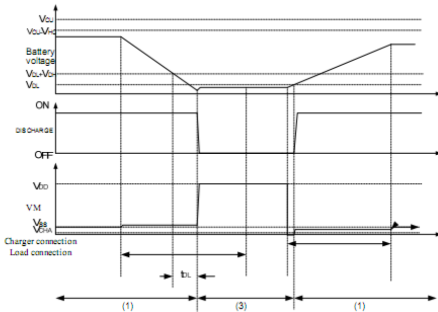
Figure5-3 Charger Detection
