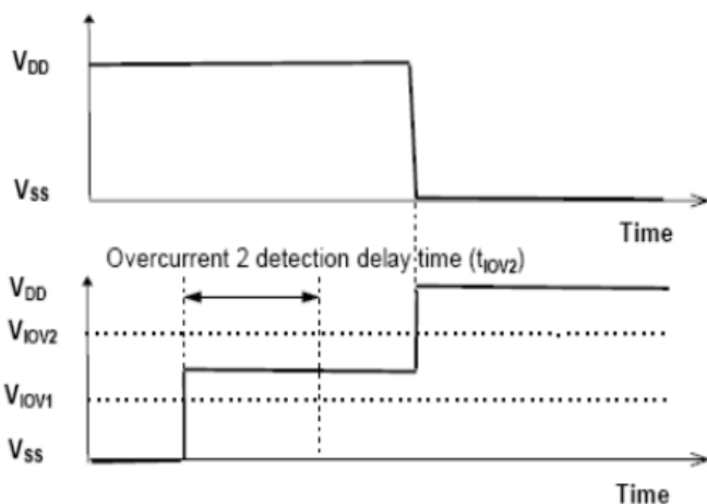
Figure 4. Overcurrent delay time
