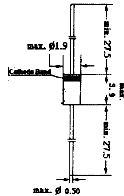
Glass case JEDEC DO-35 Dimensions in mm
