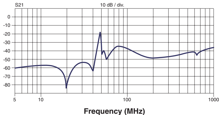
Isolation (TYP)
