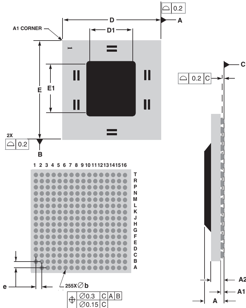
Figure 11-3. Mechanical Dimensions and Bottom Surface Nomenclature of the PC745 PBGA (ZF)
