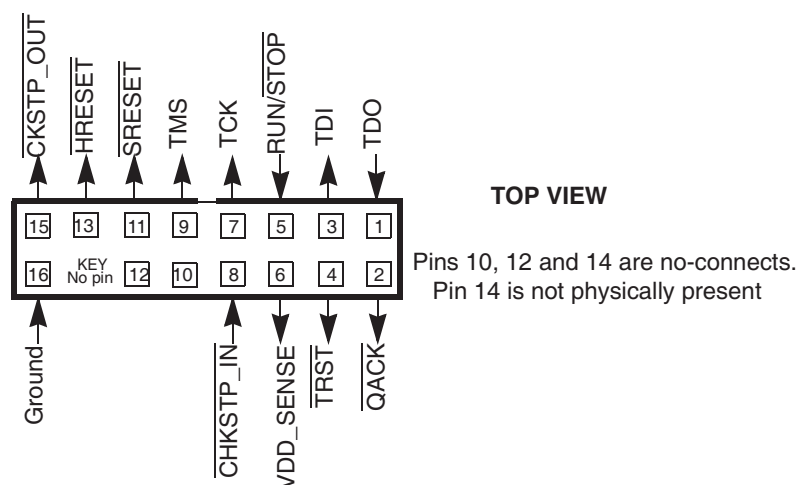
Figure 8-15. COP Connector Diagram
