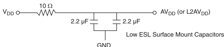
Figure 10-1. PLL Power Supply Filter Circuit
