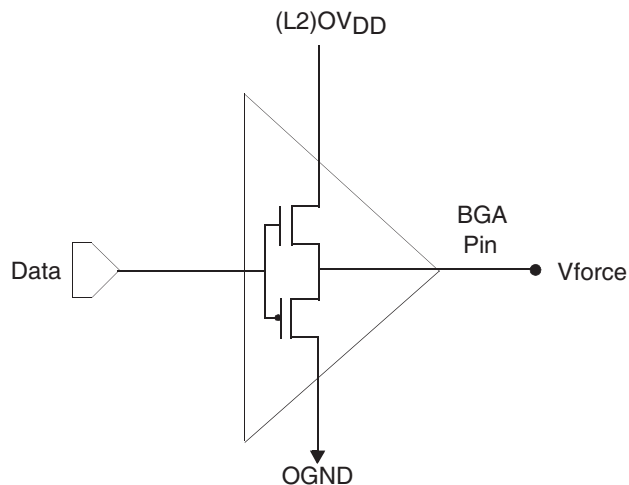
Figure 10-4. Alternate Driver Impedance Measurement Circuit
