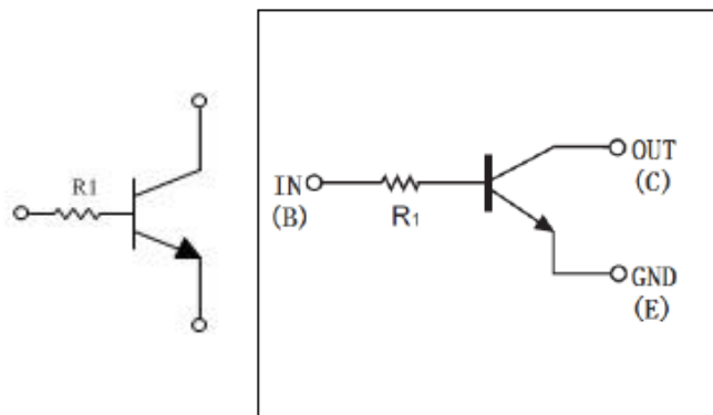
Equivalent Circuit
