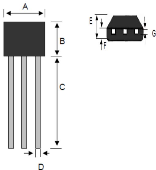
TO-92S
