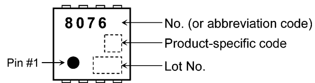
Fig. 7.1 Marking
