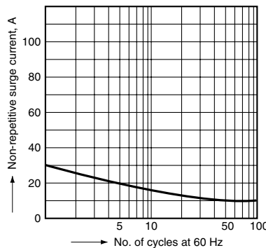
2.-(1) Characteristics of non-repetitive surge current vs. carrying time (2 A type)
