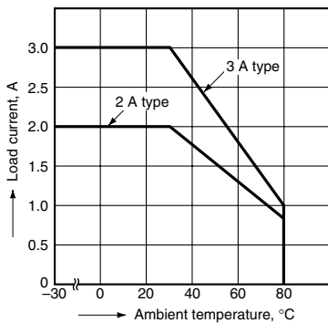
1. Characteristics of load current vs. ambient temperature Conditions: Natural cooling
