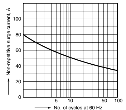
2.-(2) Characteristics of non-repetitive surge current vs. carrying time (3 A type)
