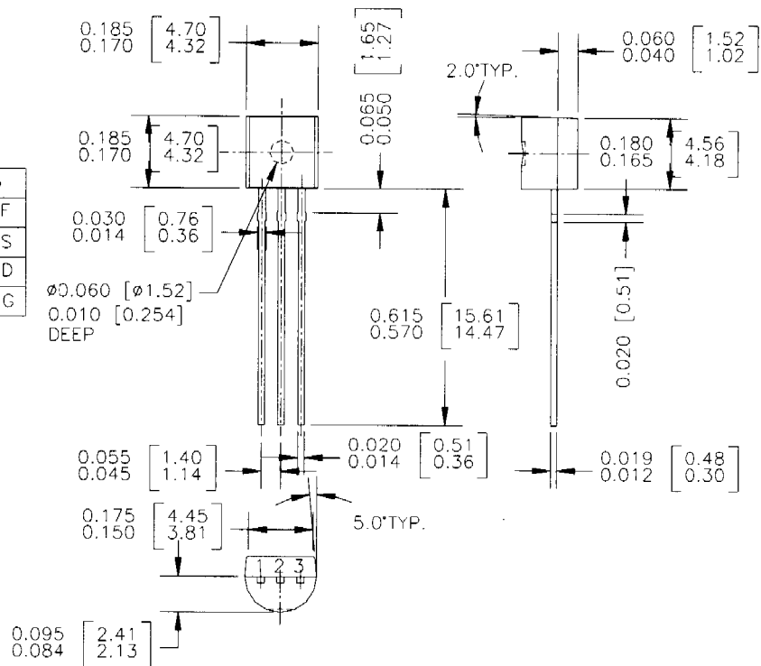
TO-92 (92,94,96)
