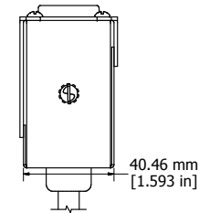
ASSEMBLY - VIEW FROM SIDE
