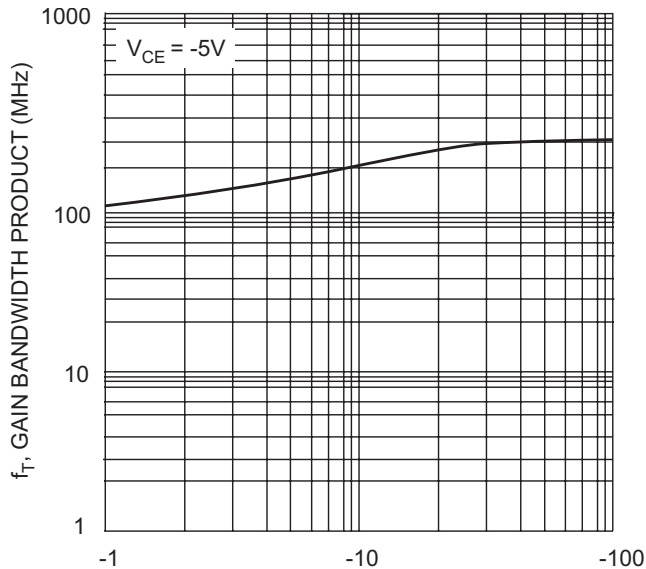
I_C , COLLECTOR CURRENT (mA)
