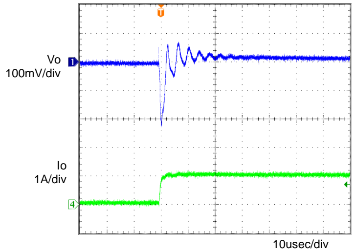
Figure 4. Transient Response (0→1.0A) C_o=1\mu F, T_a=25^\circ\text{C}
