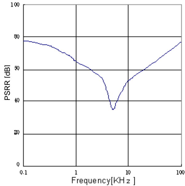
Figure 32. PSRR ( I_o=0\text{mA} )
