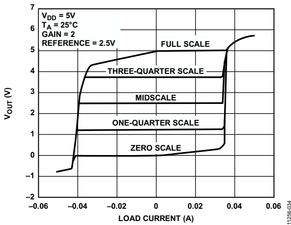
Figure 33. Source and Sink Capability at 5 V, Gain = 2
