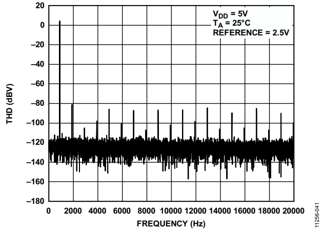
Figure 40. Total Harmonic Distortion at 1 kHz
