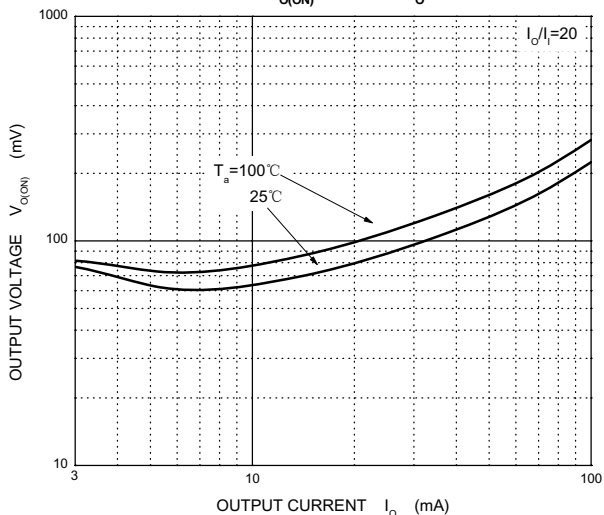
V_{oi(on)} — I_o
