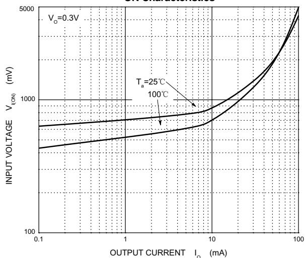
ON Characteristics
