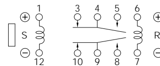
Double coil latch type (reset position)
