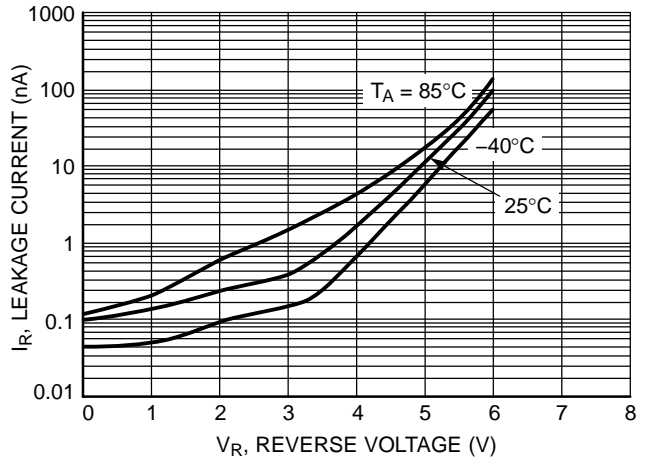
Figure 6. Leakage Current versus Reverse Voltage
