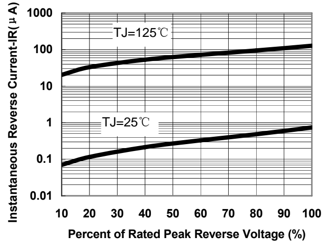
Fig.2-Typical Reverse Characteristics
