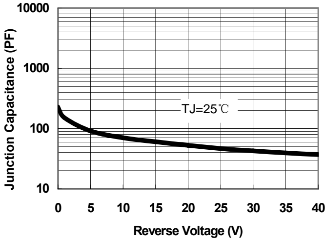
Fig.1-Typical Junction Capacitance
