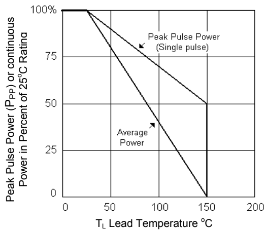
FIGURE 4 Derating Curve
