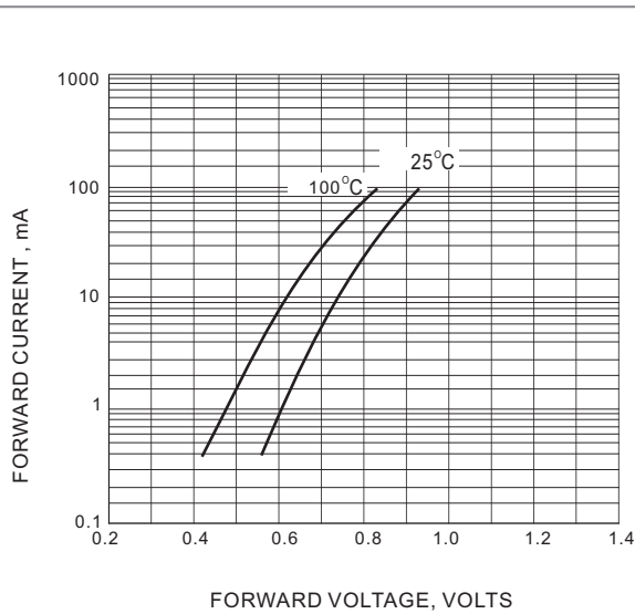
FIG. 1-TYPICAL FORWARD CHARACTERISTIC
