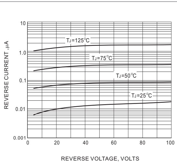
FIG. 2-TYPICAL REVERSE CHARACTERISTICS
