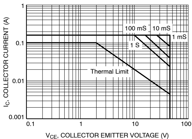
Figure 34. Safe Operating Area for LBC847A, LBC847B, LBC847C, LBC850B, LBC850C
