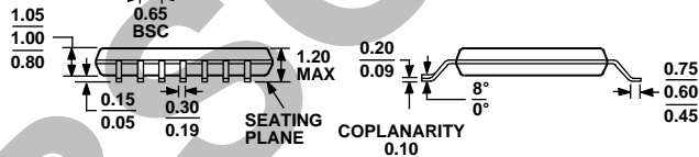
Figure 22. 14-Lead Thin Shrink Small Outline Package [TSSOP] (RU-14) Dimensions shown in millimeters
