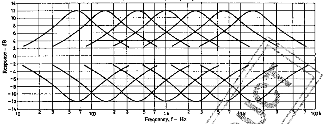
STK301-060A Frequency response
