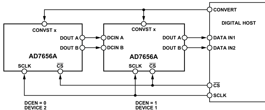
Figure 29. Daisy-Chain Configuration
