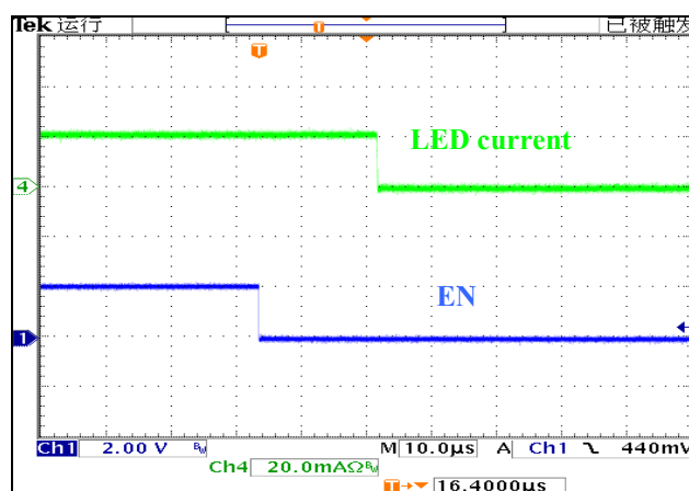
Fig. 2 Shutdown from EN pin
