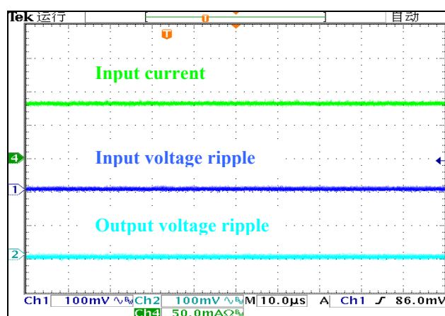
Fig. 4 Operating at 1x mode with 100% brightness
