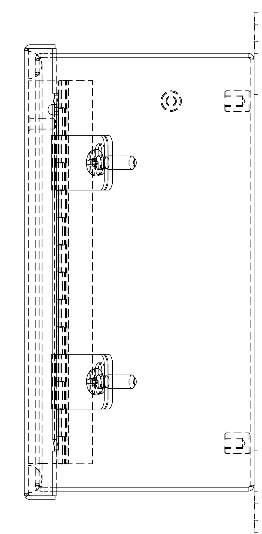
SIDE VIEW
