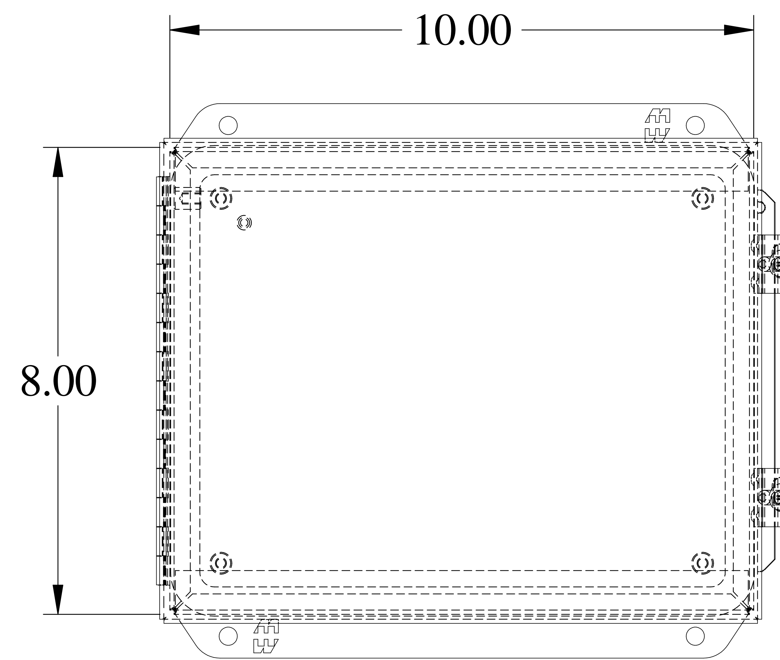
FRONT VIEW
