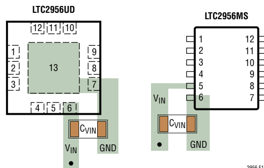
Figure 19. Recommended Layout for the V_{\text{IN}} Bypass Capacitor
