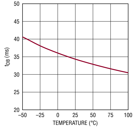
PB Debounce Time vs Temperature
