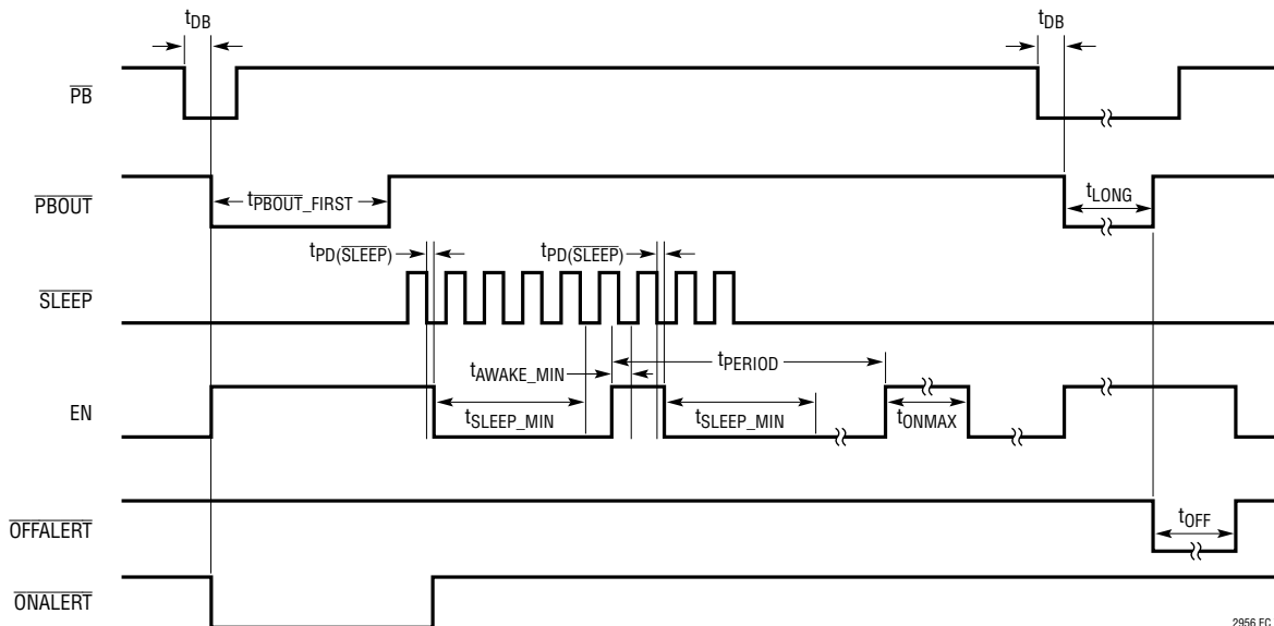
Timing Diagram
