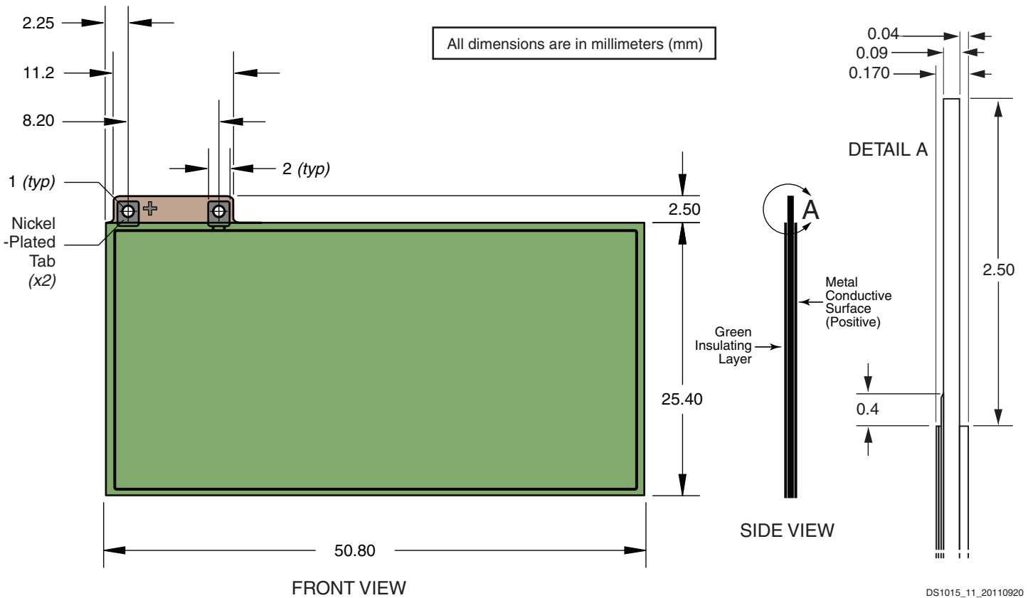
Figure 11: Front and Side Views
