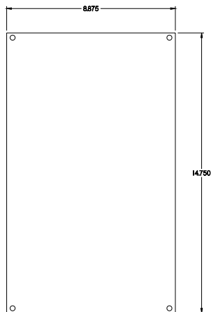
INNER PANEL
