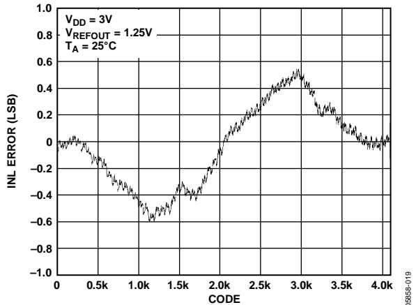
Figure 18. INL—AD5623R-3
