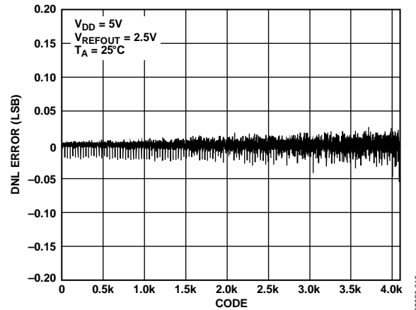
Figure 15. DNL—AD5623R-5
