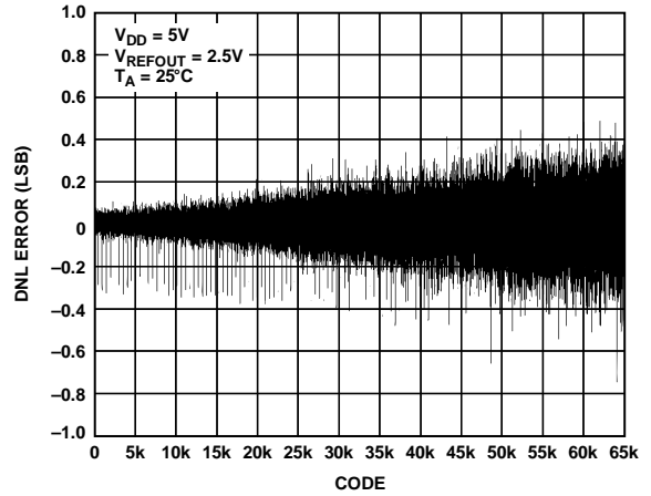
Figure 13. DNL—AD5663R-5
