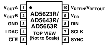
Figure 3. Pin Configuration
