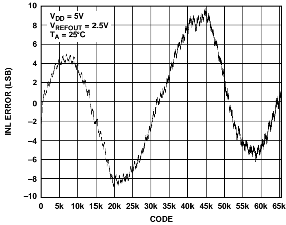
Figure 10. INL—AD5663R-5
