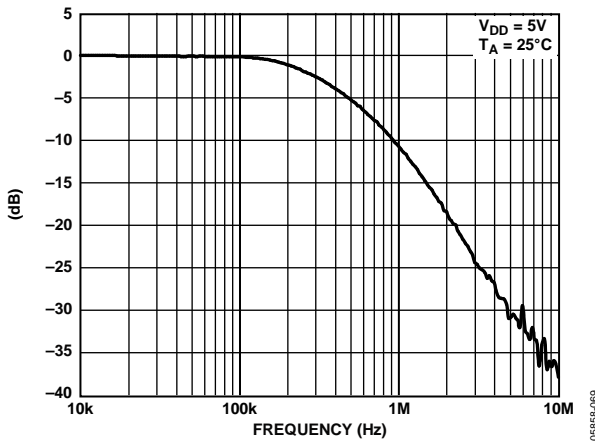
Figure 47. Multiplier Bandwidth
