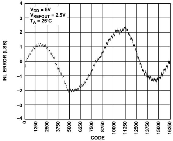
Figure 11. INL—AD5643R-5
