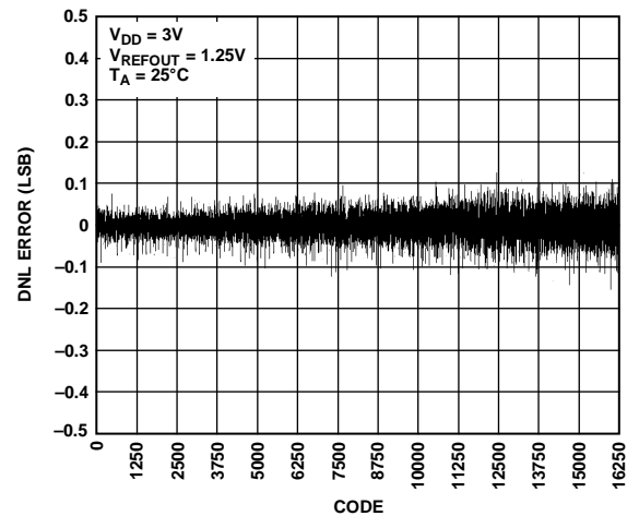
Figure 20. DNL—AD5643R-3
