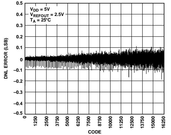
Figure 14. DNL—AD5643R-5
