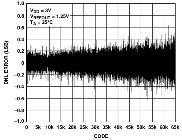
Figure 19. DNL—AD5663R-3
