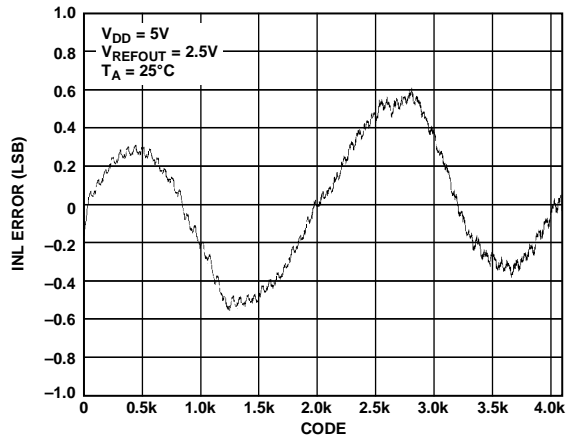
Figure 12. INL—AD5623R-5
