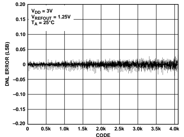
Figure 21. DNL—AD5623R-3
