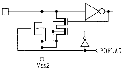
Figure 3 S1 to S4 and M1 to M4 Input Circuits
