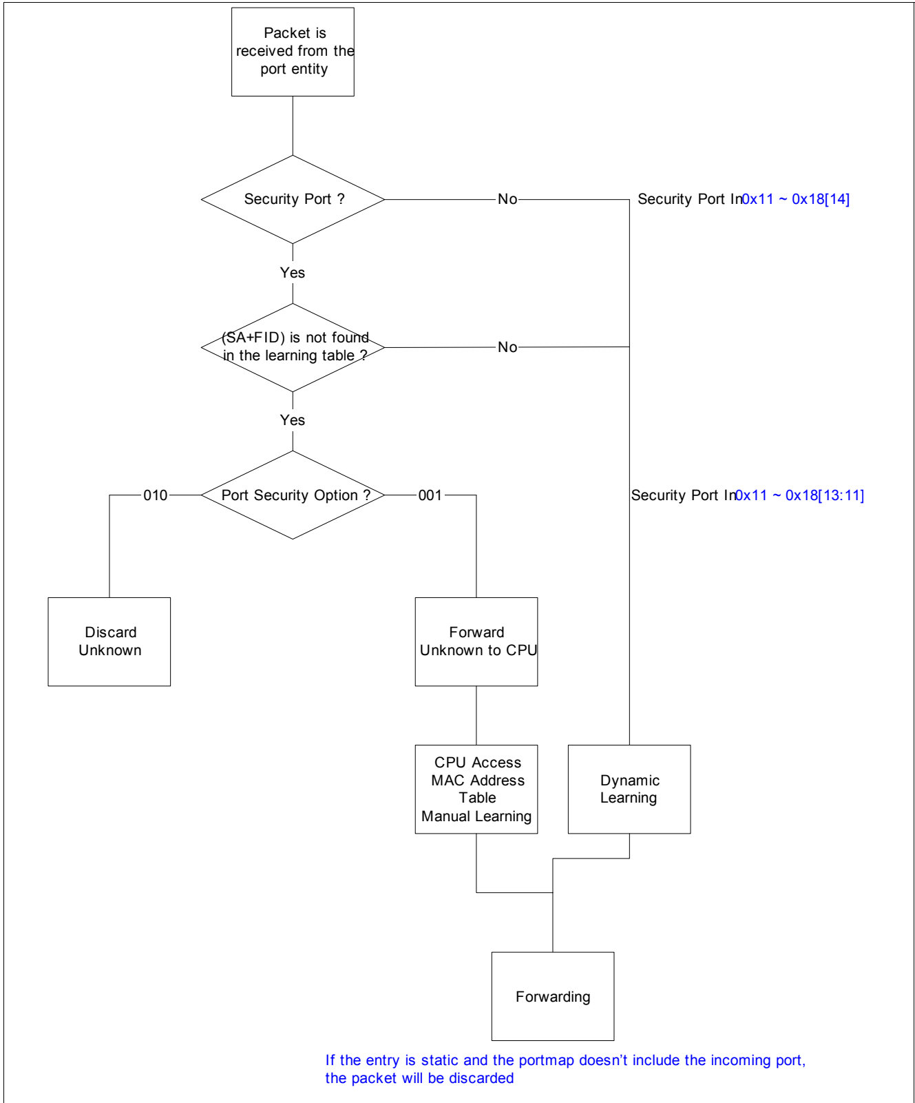
Figure 6 Flow chart of 802.1x Security Function
