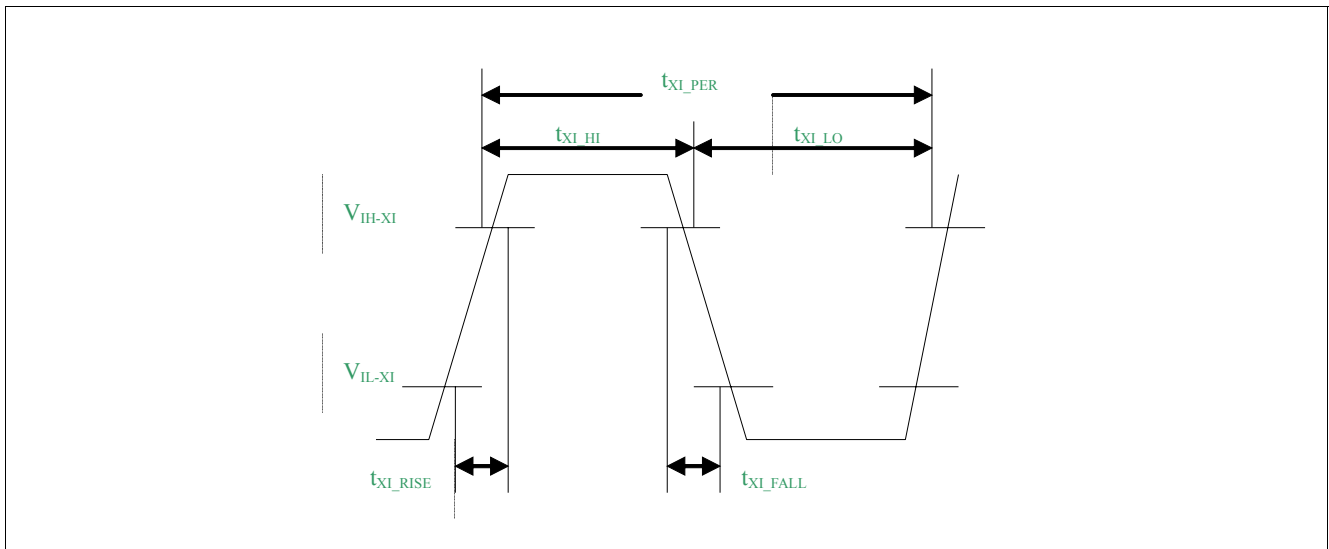
Figure 20 XTAL/OSC Timing
