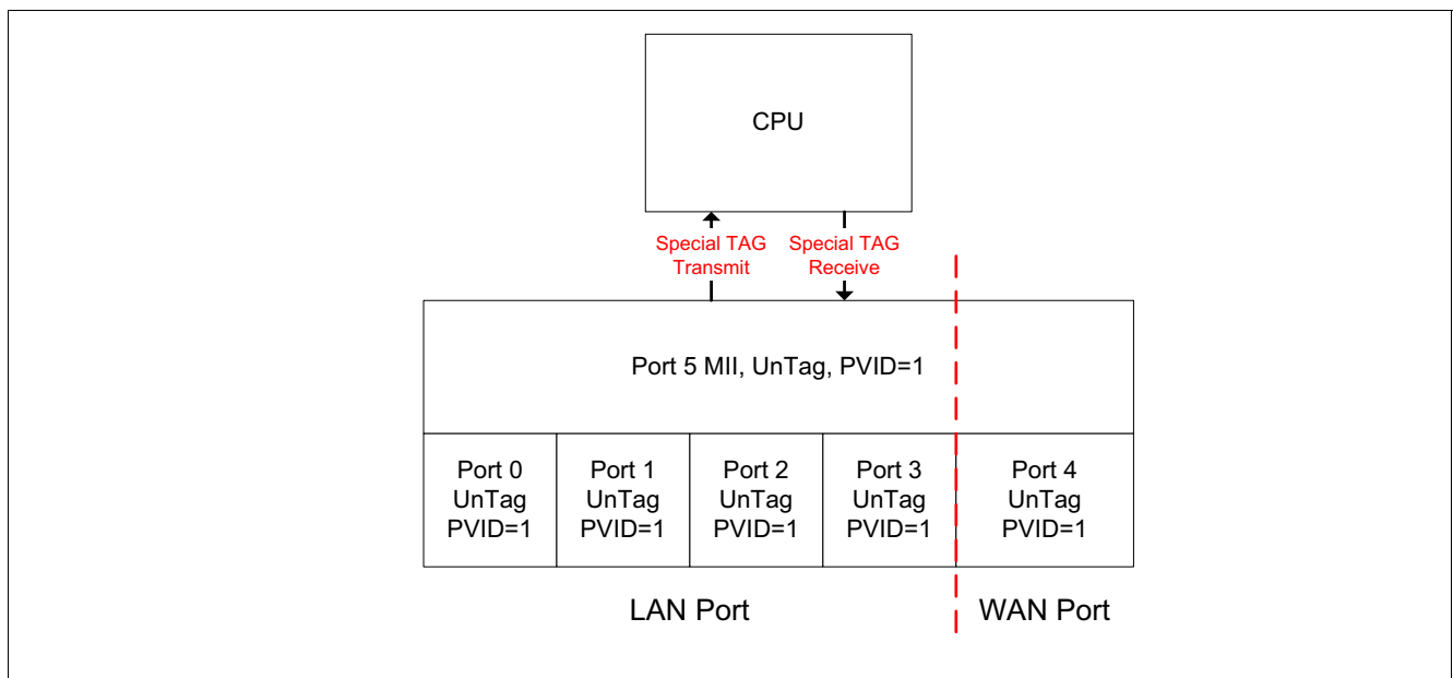
Figure 8 The configurations of the implementation by ADM6996M/MX Special TAG functions
