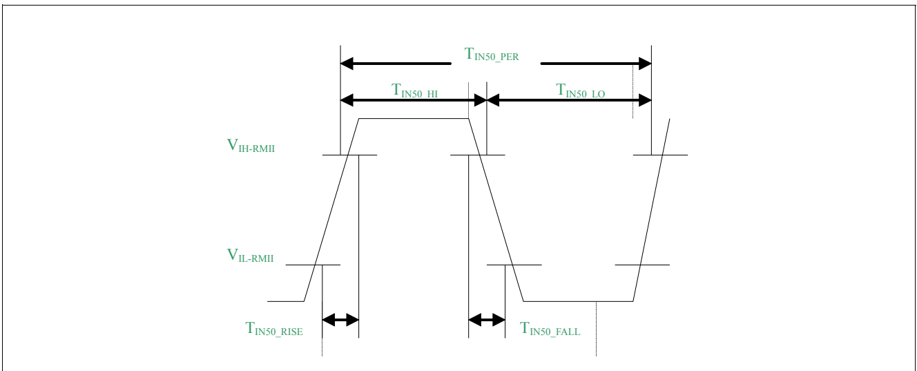
Figure 27 RMII REFCLK Input Timing
