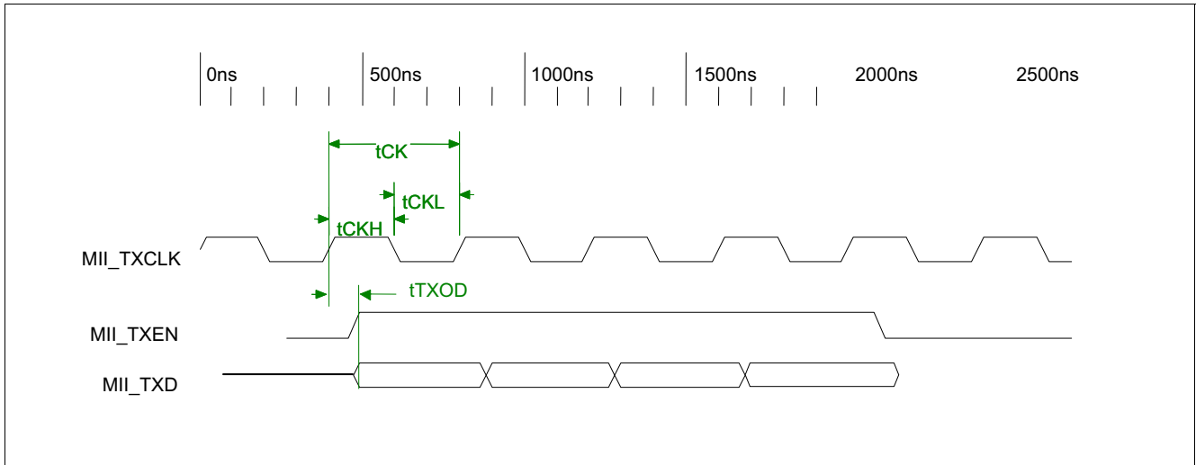
Figure 24 10Base-TX MII Output Timing
