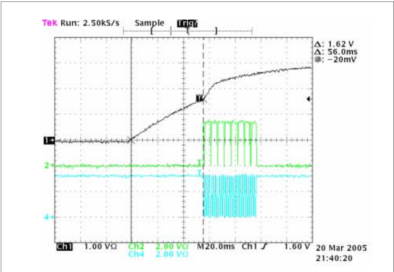
Figure 15 Timing Diagram of RC, EECS and EESK (with correct signature EEPROM)
