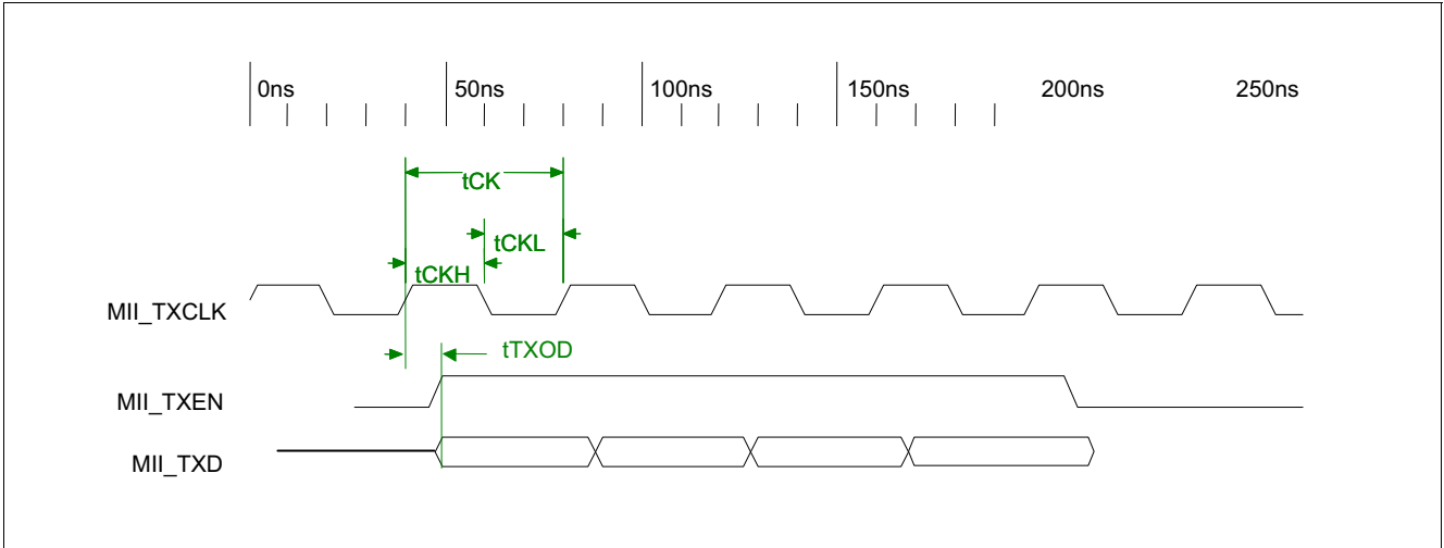
Figure 26 100Base-TX MII Output Timing
