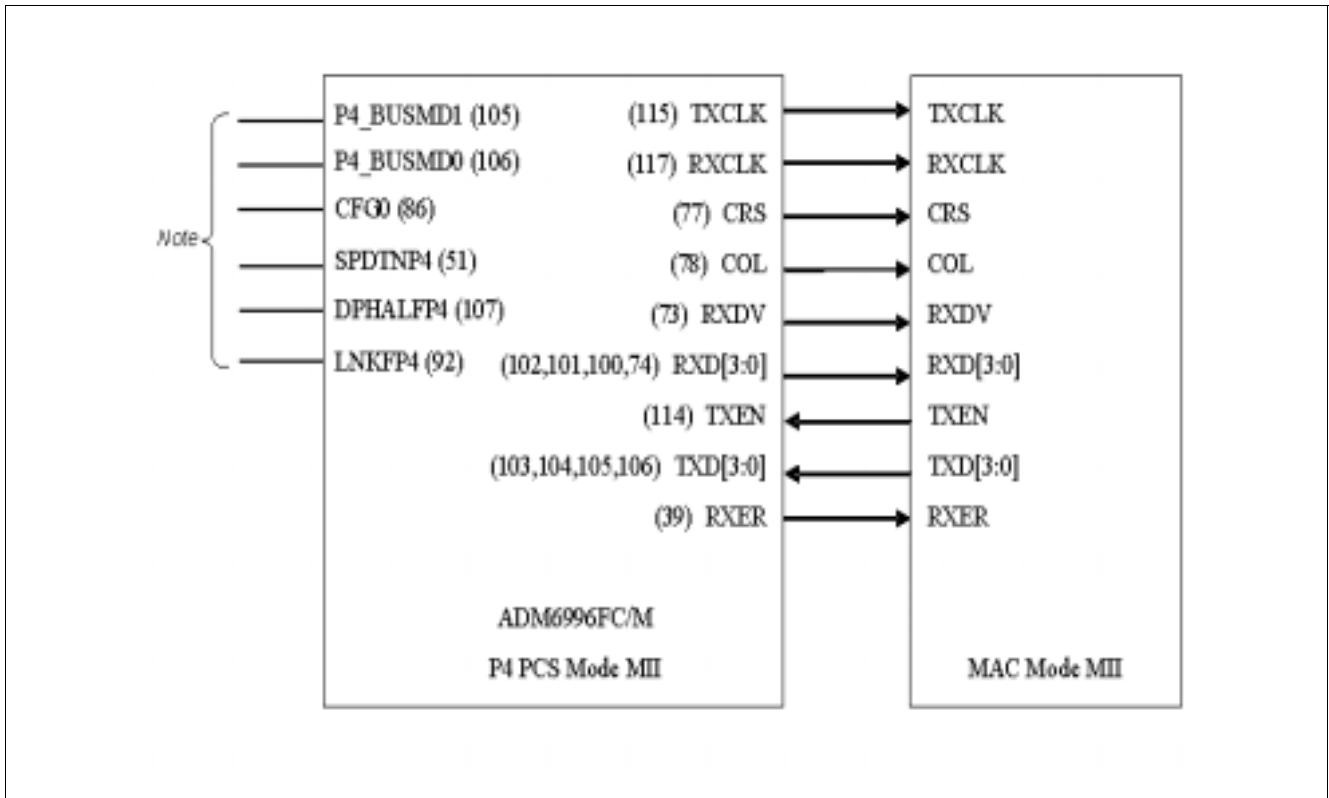
Figure 11 100M Full duplex MAC to MAC MII Connection
