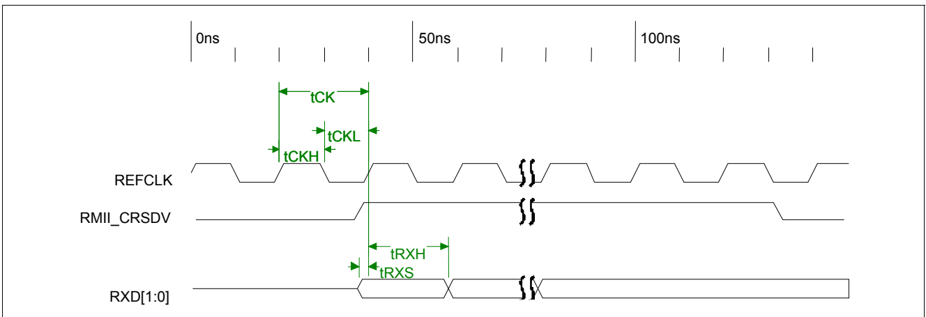
Figure 30 Reduce MII Timing (2 of 2)
