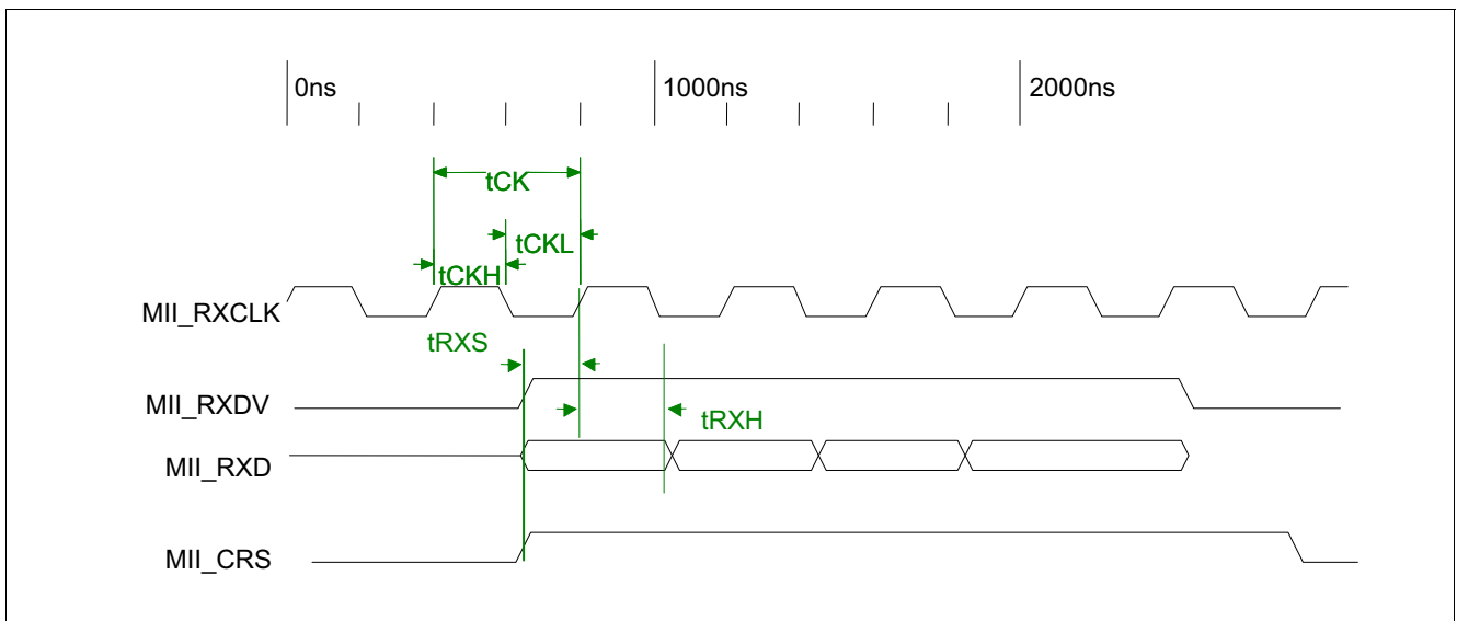
Figure 23 10Base-TX MII Input Timing
