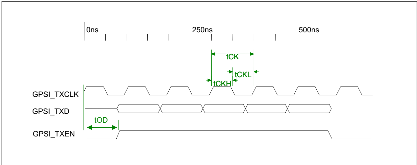
Figure 32 GPSI (7-wire) Output Timing
