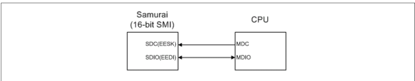
Figure 17 SMI Interface
