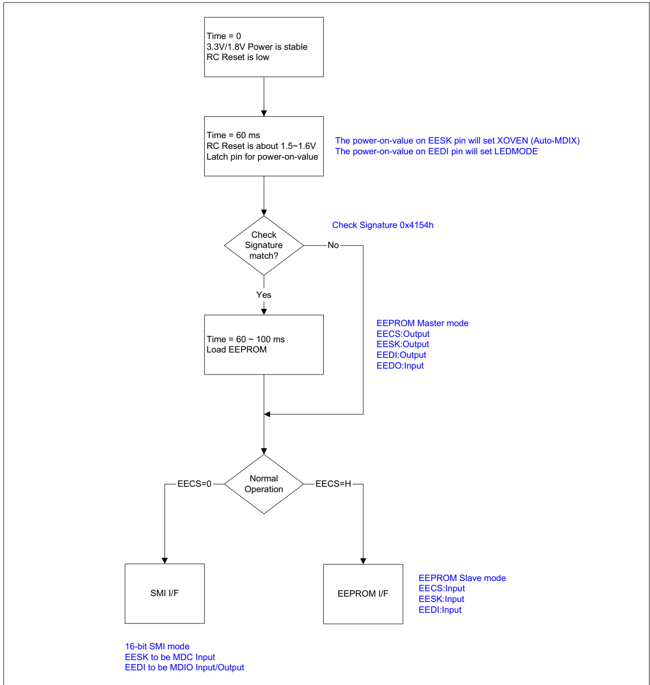
Figure 14 The Power-On-Sequence of Samurai
