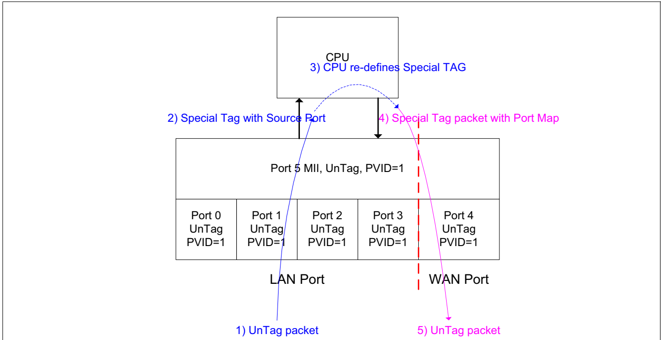
Figure 9 Software Operation
