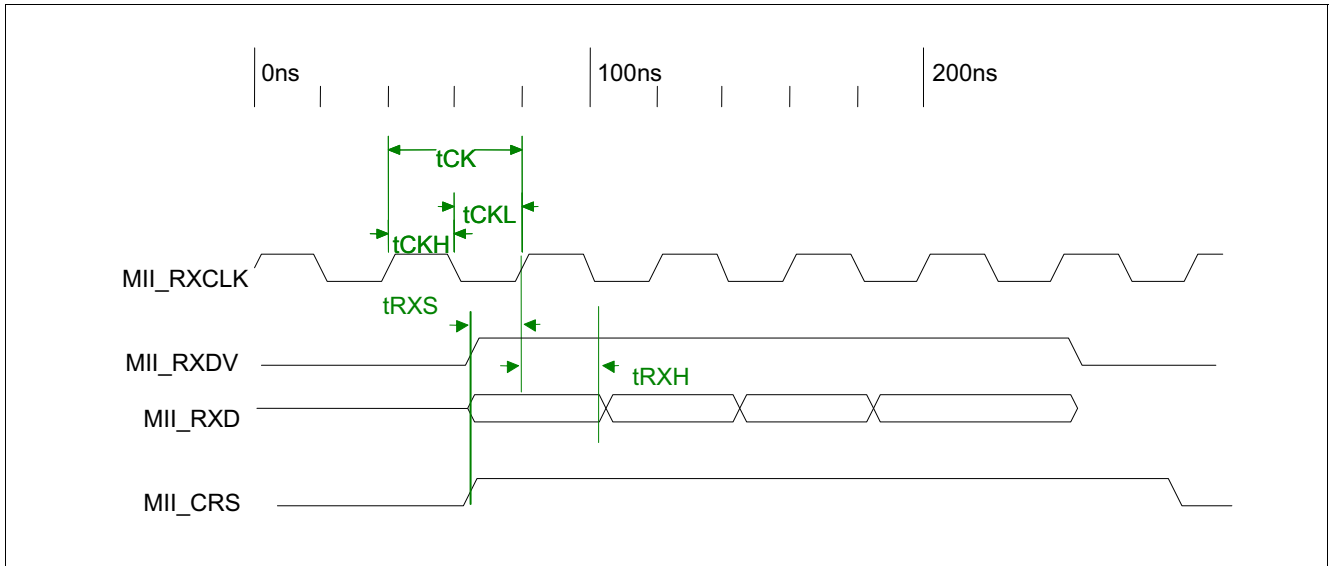
Figure 25 100Base-TX MII Input Timing
