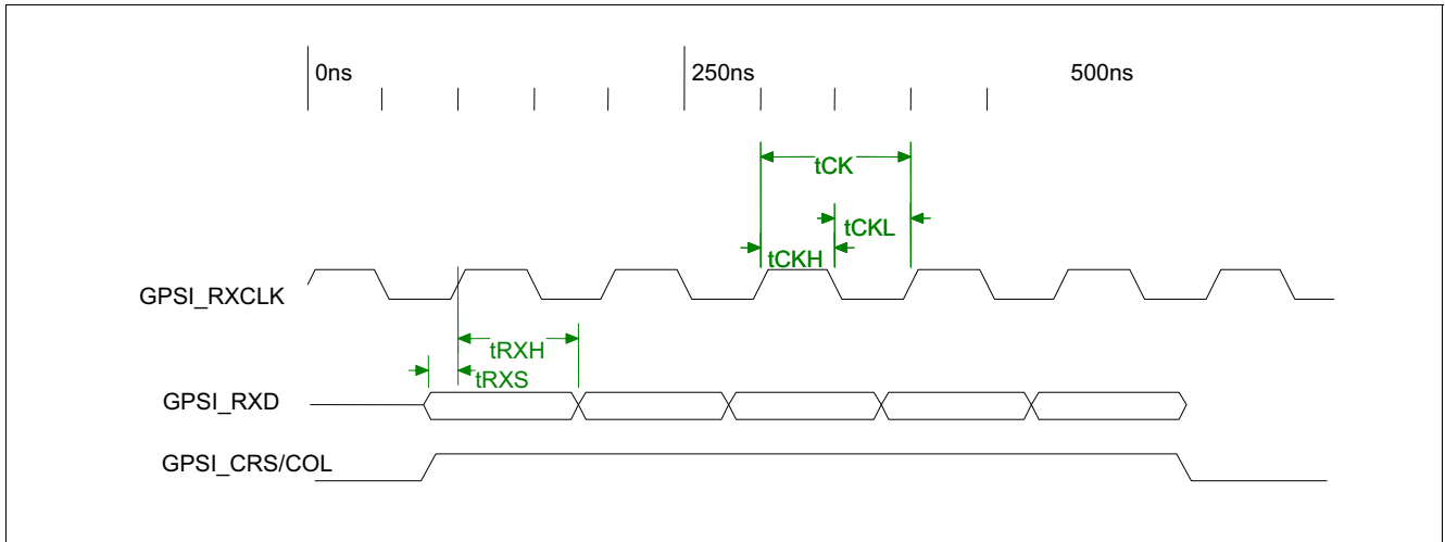
Figure 31 GPSI (7-wire) Input Timing
