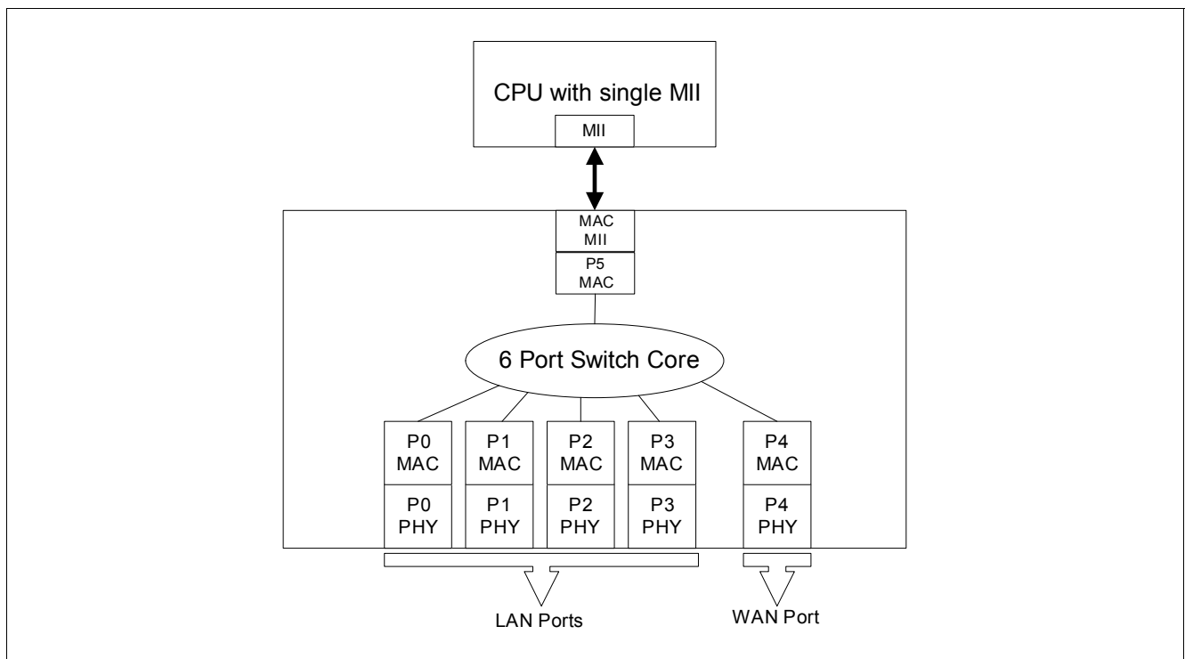
Figure 7 ADM6996M/MX to CPU with single MII Connection
