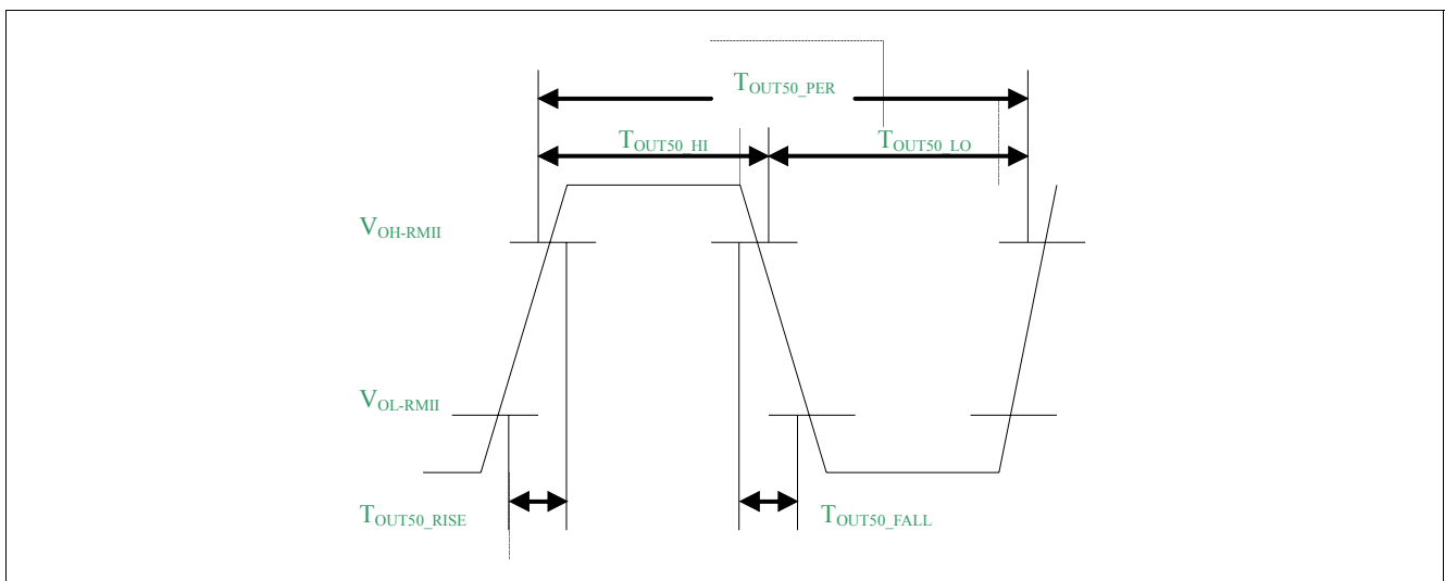
Figure 28 RMI REFCLK Output Timing
