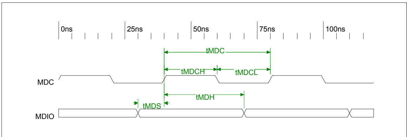
Figure 34 MDC/MDIO Timing
