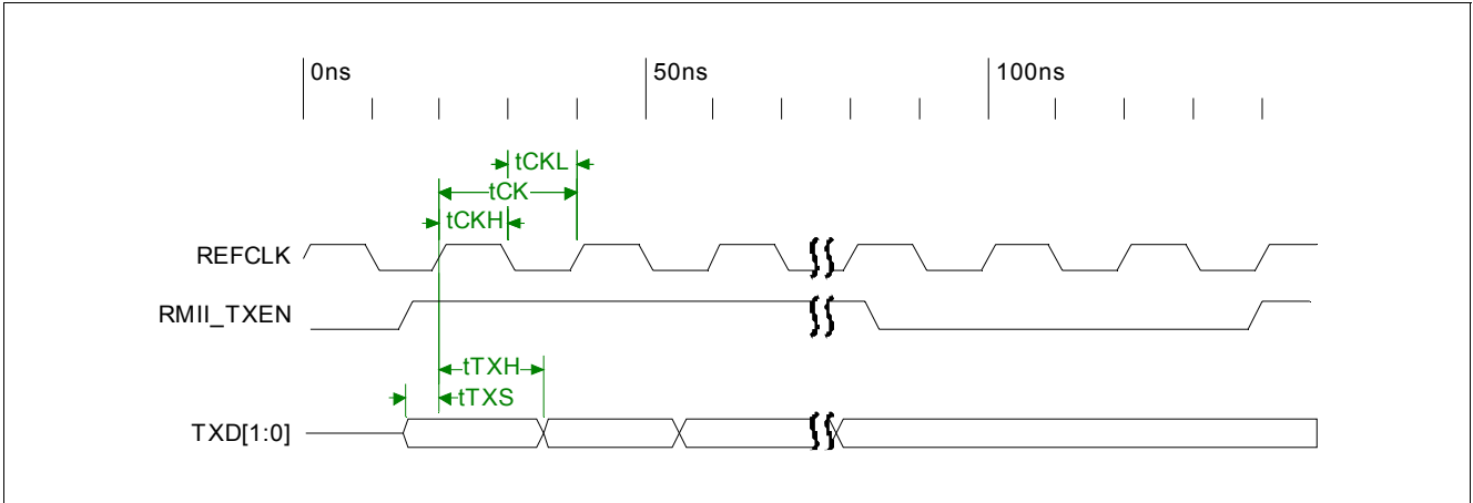
Figure 29 Reduce MII Timing (1 of 2)
