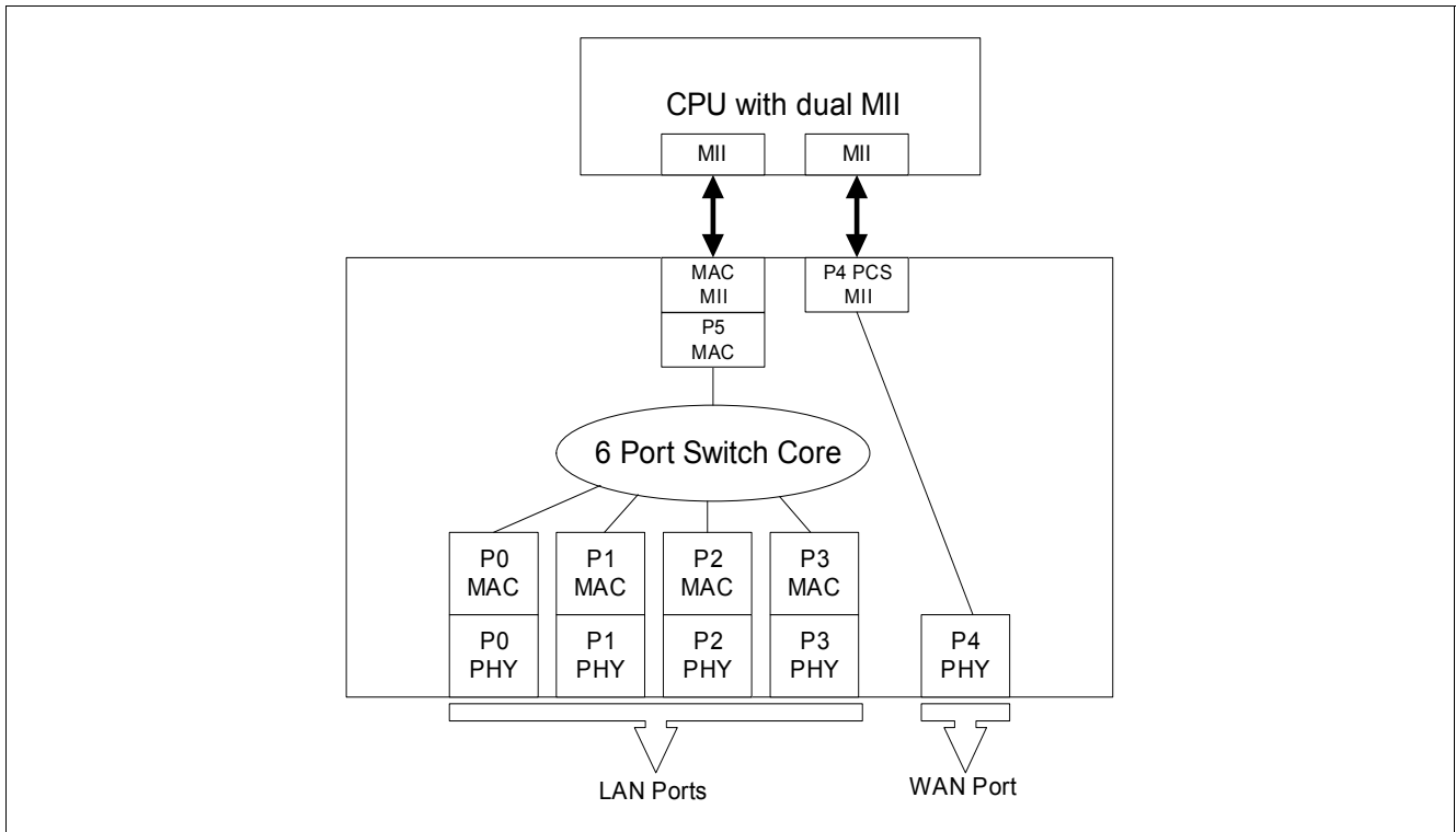
Figure 10 ADM6996M/MX to CPU with dual MII Connection
