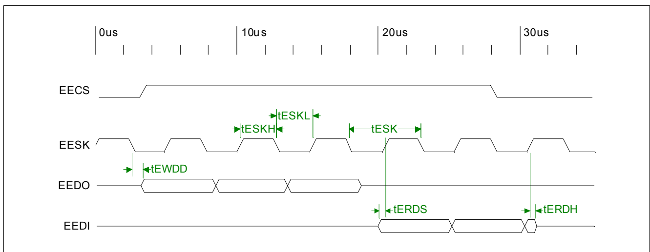
Figure 22 EEPROM Interface Timing
