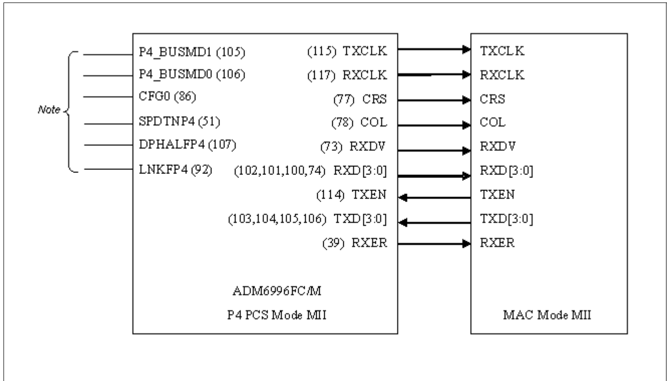
Figure 12 PCS to MAC MII connection
