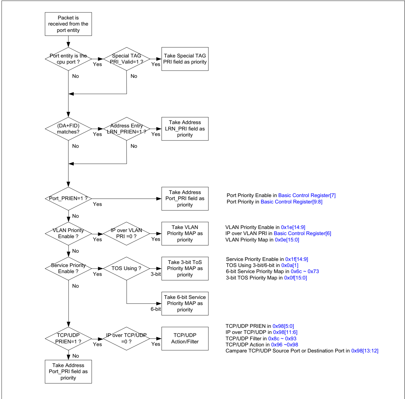
Figure 5 To Configure Samurai QoS function
