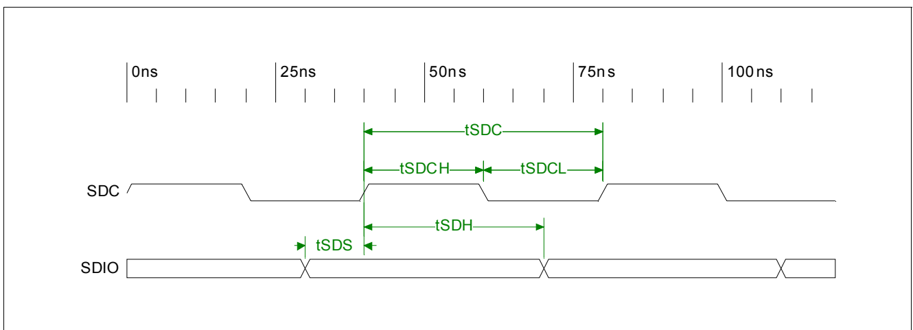
Figure 33 SDC/SDIO Timing
