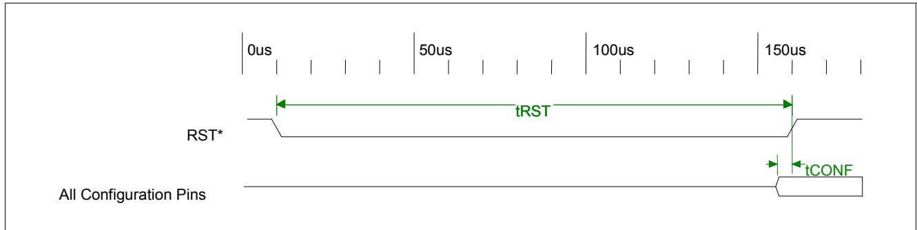
Figure 21 Power On Reset Timing
