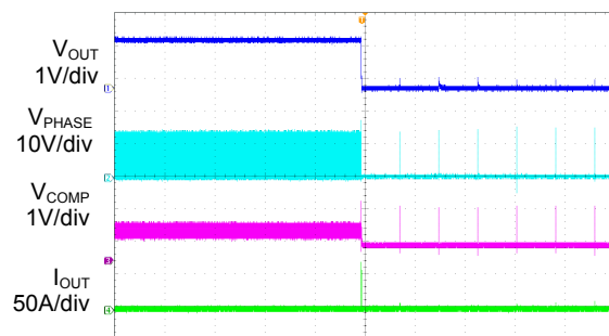
Time 10ms/div
