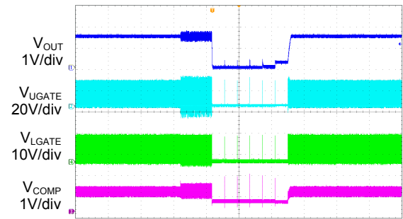
Time 20ms/div
