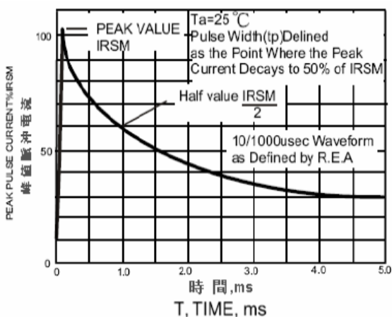
FIG.5–脉冲额定曲线 FIG.5–PULSE RATING CURVEE
