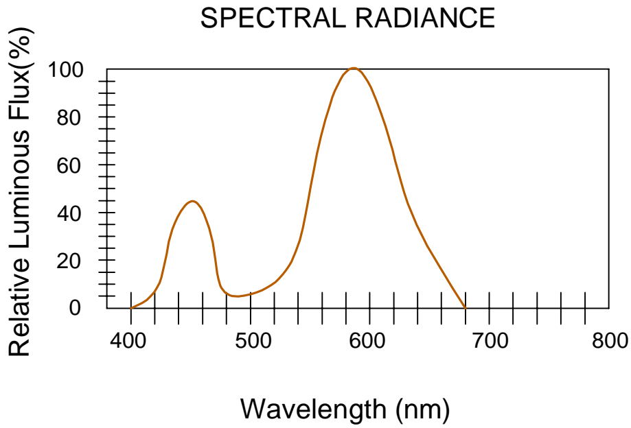
Fig.5 Luminous Spectrum(Ta=25 °C)
