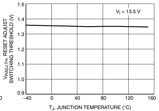
Figure 29. Reset Adjust Switching Threshold vs. Junction Temperature
