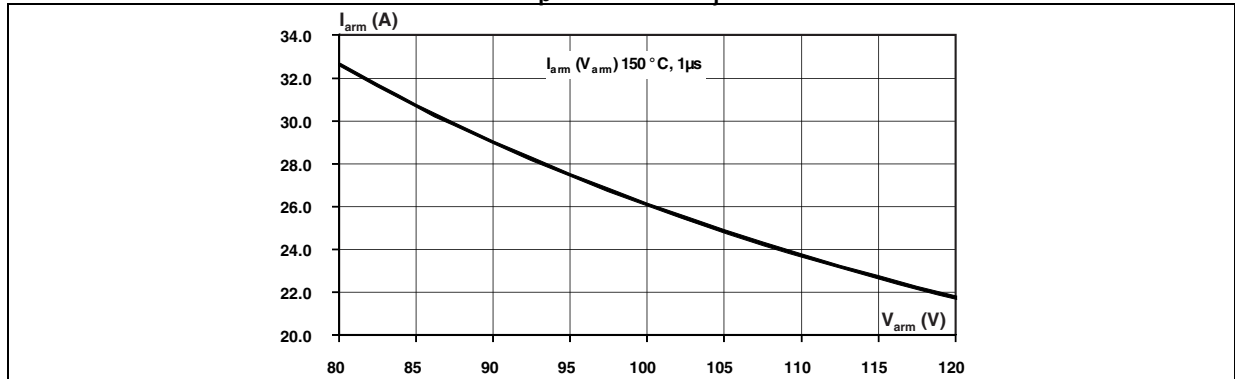
Figure 14. Reverse safe operating area ( t_p < 1\ \mu\text{s} and T_j < 150^\circ\text{C} )
