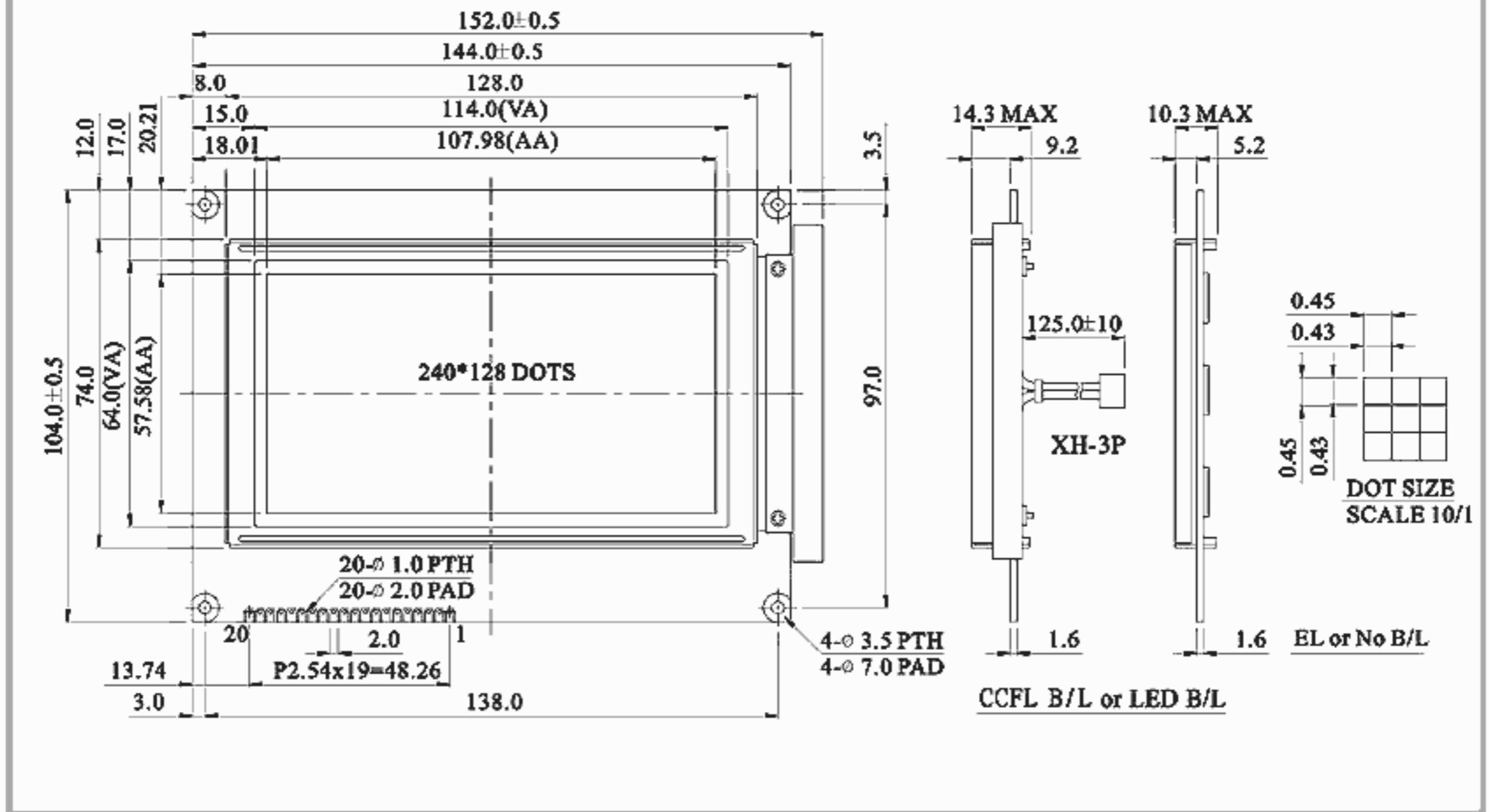
Dimension drawing
