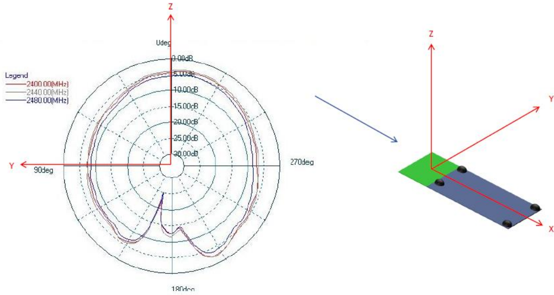
Figure 11: Radiation pattern of BLE121LR when mounted to the DKBLE
