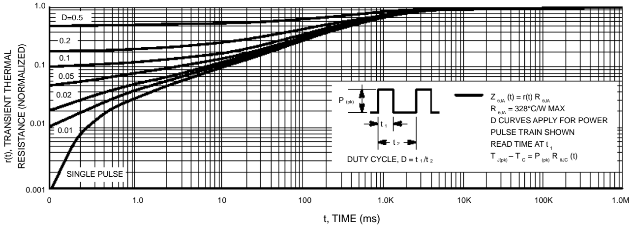
Figure 11. Thermal Response
