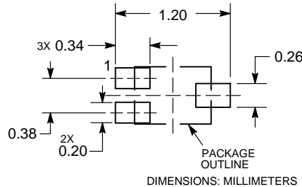
DIMENSIONS: MILLIMETERS
