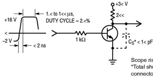
Figure 1. Turn-On Time
