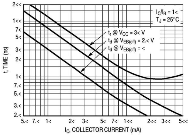
Figure 5. Turn-On Time
