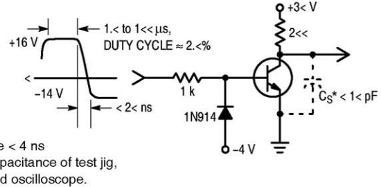
Figure 2. Turn-Off Time
