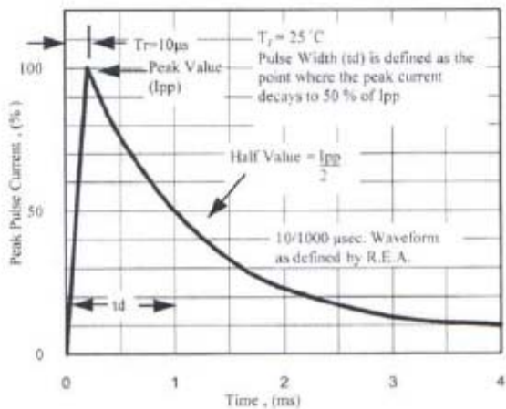
Fig. 5 - Pulse Waveform
