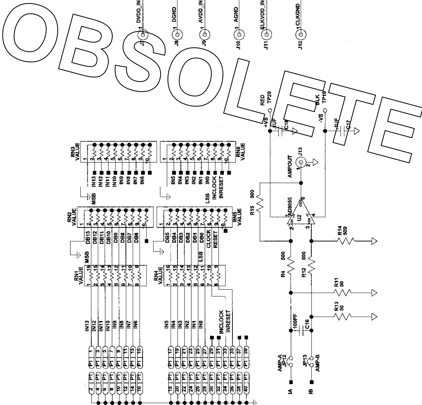
Figure 54. Drafting Schematic of Evaluation Board
